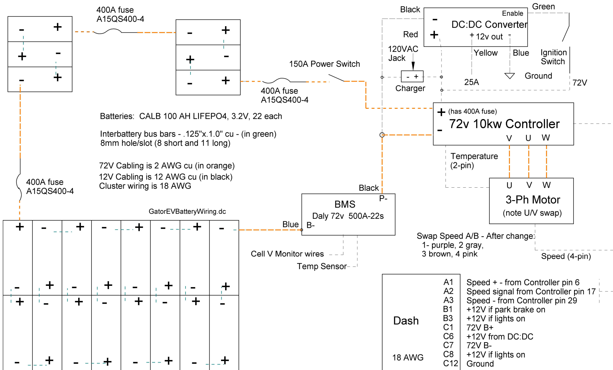
Gator EV Power Wiring Diagram
